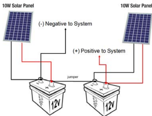
Two 10 watt 12v solar panels charging two 12v batteries in a 24v configuration
