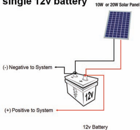
Single 10 watt 12v solar panel charging a single 12v battery
